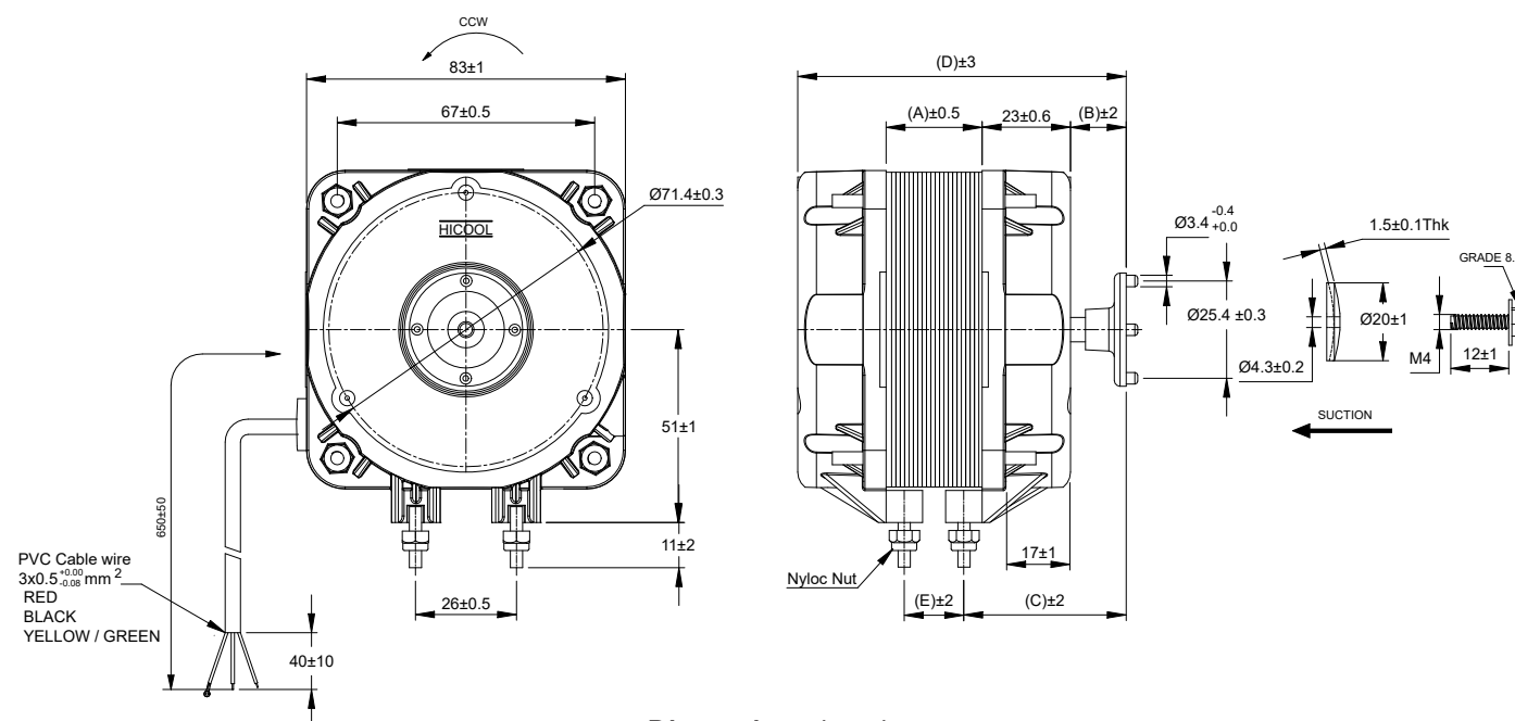
Dimensions (mm)
